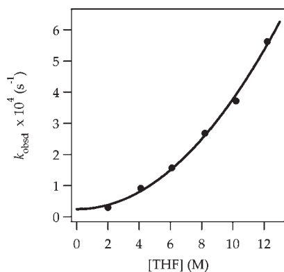
Figure 10. Plot of k_{\text{obsd}} versus [\text{THF}] in hexanes for the ortholithiation of 1-2,6- d_2 (0.002 M) by LDA (0.050 M) at -65\text{ }^\circ\text{C} measured by ^{19}\text{F} NMR spectroscopy. The curve depicts an unweighted least-squares fit to y = k[\text{THF}]^n + c . [ k = (3 \pm 1) \times 10^{-6} , n = 2.0 \pm 0.2 , and c = (3 \pm 1) \times 10^{-5} .]
