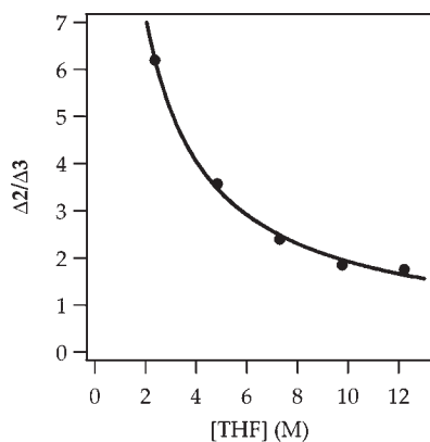
Figure 8. Ratio of relative initial rates of formation of 2 and 3 , ( \Delta 2/\Delta t )/( \Delta 3/\Delta t ), versus [THF] in hexanes for the ortholithiation of 1 (0.050 M) by LDA (0.10 M) at -65\text{ }^\circ\text{C} measured by ^{19}\text{F} NMR spectroscopy. The elevated temperature was used to shorten the duration of the experiments. The curve depicts an unweighted least-squares fit to y = a[\text{THF}]^n + b . [ a = 12.5 \pm 0.8 , n = -0.8 \pm 0.2 , and b = 0.1 \pm 0.8 .]
