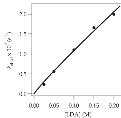
Figure 9. Plot of k_{\text{obsd}} versus [LDA] in THF (12.2 M) for the ortholithiation of 1-2,6- d_2 (0.002 M) at -65\text{ }^\circ\text{C} measured by ^{19}\text{F} NMR spectroscopy. The curve depicts an unweighted least-squares fit to y = k[\text{LDA}]^n . [ k = (9 \pm 1) \times 10^{-3} , n = 0.92 \pm 0.06 .]
