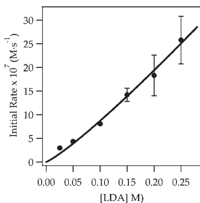
Figure 5. Plot of initial rate versus [LDA] in THF (12.2 M) for the ortholithiation of 1 (0.050 M) at -78\text{ }^{\circ}\text{C} measured by IR spectroscopy. The curve depicts an unweighted least-squares fit to y = a[\text{LDA}]^n . [ a = (1.2 \pm 0.2) \times 10^{-5} , n = (1.16 \pm 0.09) .]
