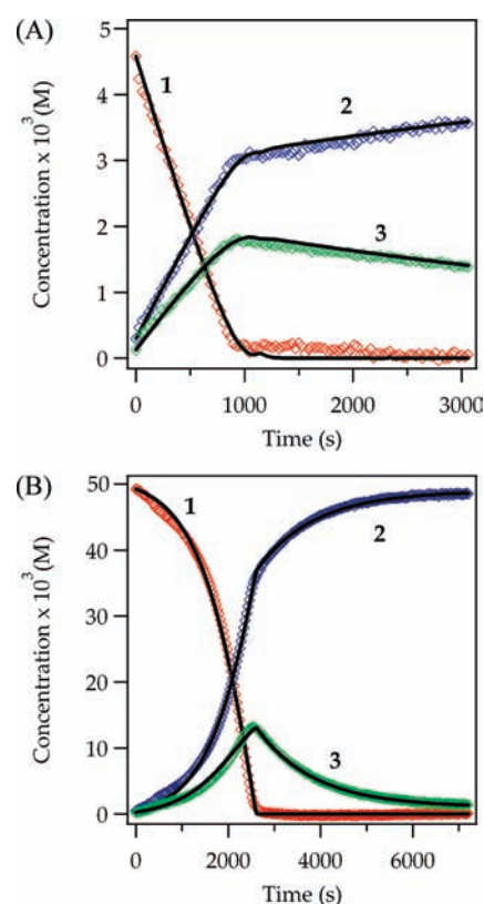
Figure 1. Representative plots of concentration versus time monitored by ^{19}\text{F} NMR spectroscopy for the ortholithiation of 1 and formation of 2 and 3 by LDA (0.10 M) in THF (12.2 M) at -60\text{ }^\circ\text{C} : (A) 0.005 M 1 ; (B) 0.050 M 1 . The curves represent best-fit numerical integrations as described below.
